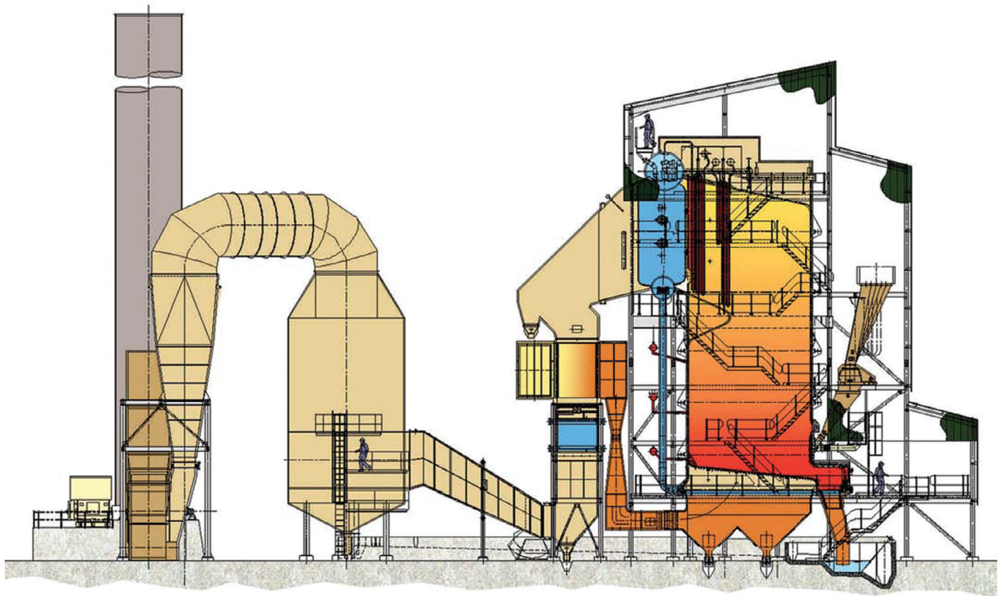
Typical bagasse fired boiler with pinhole grate.
