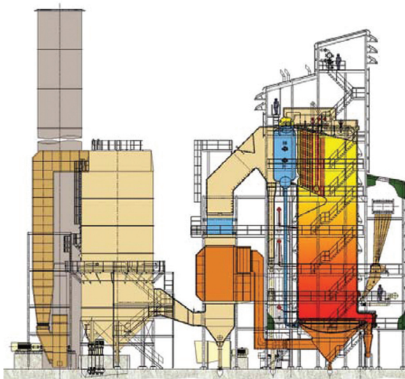
160 T Bidrum 45 Bar bagasse and woodwaste fired boiler.
