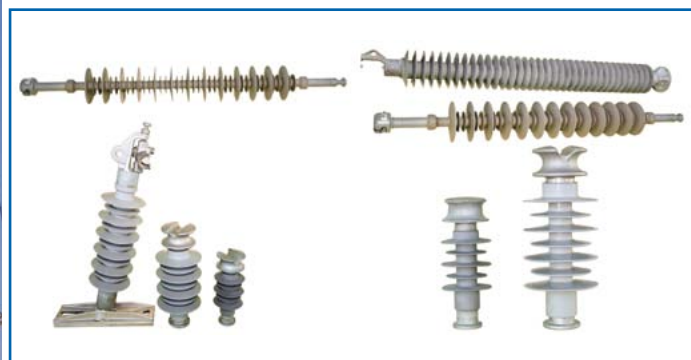
Composite Long Rod & Line Post Insulators
